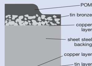
Cross section of SKF POM Composite
