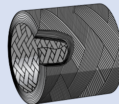
Cross section of SKF Filament Wound
